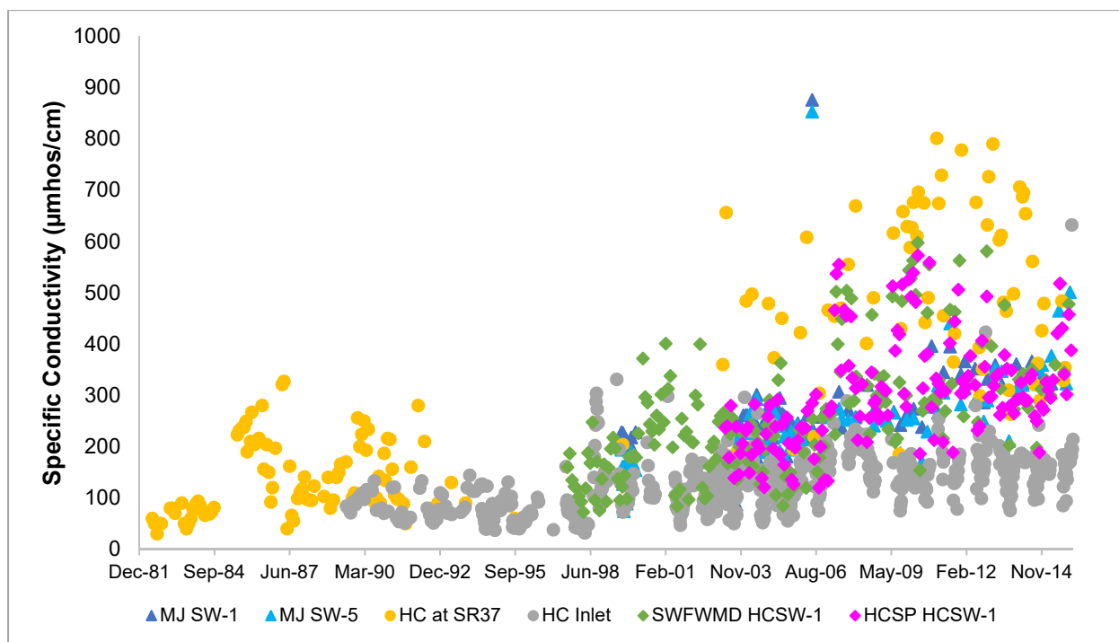
Figure I-31. Specific conductivity collected in West Fork Horse Creek (MJ SW-1 and SW-5), Horse Creek upstream of NPDES discharges (HC at 37 and HC Inlet), and at HCSW-1 (HCSP and SWFWMD) from 1982 to 2015.
