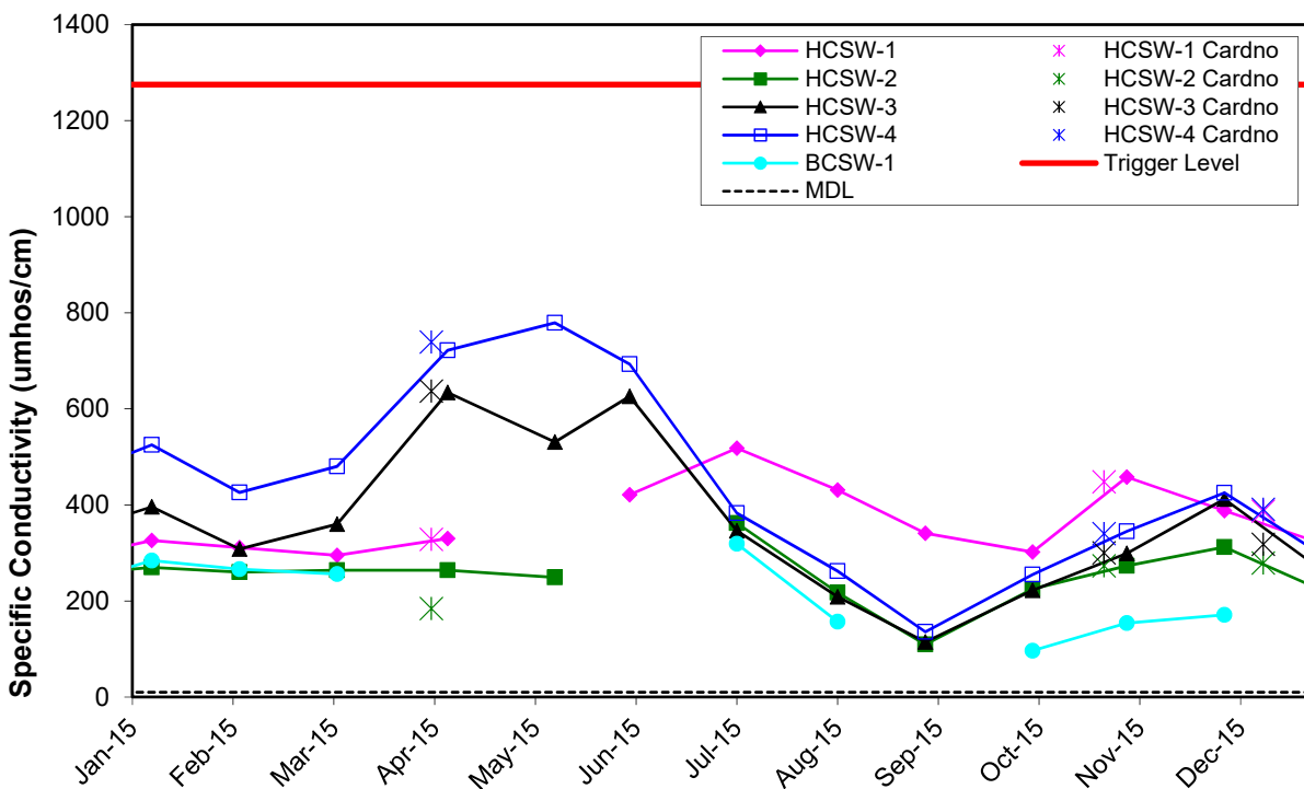
Figure 6-16. Specific conductivity measurements obtained during monthly HCSP water quality sampling and biological sampling events in 2015.
