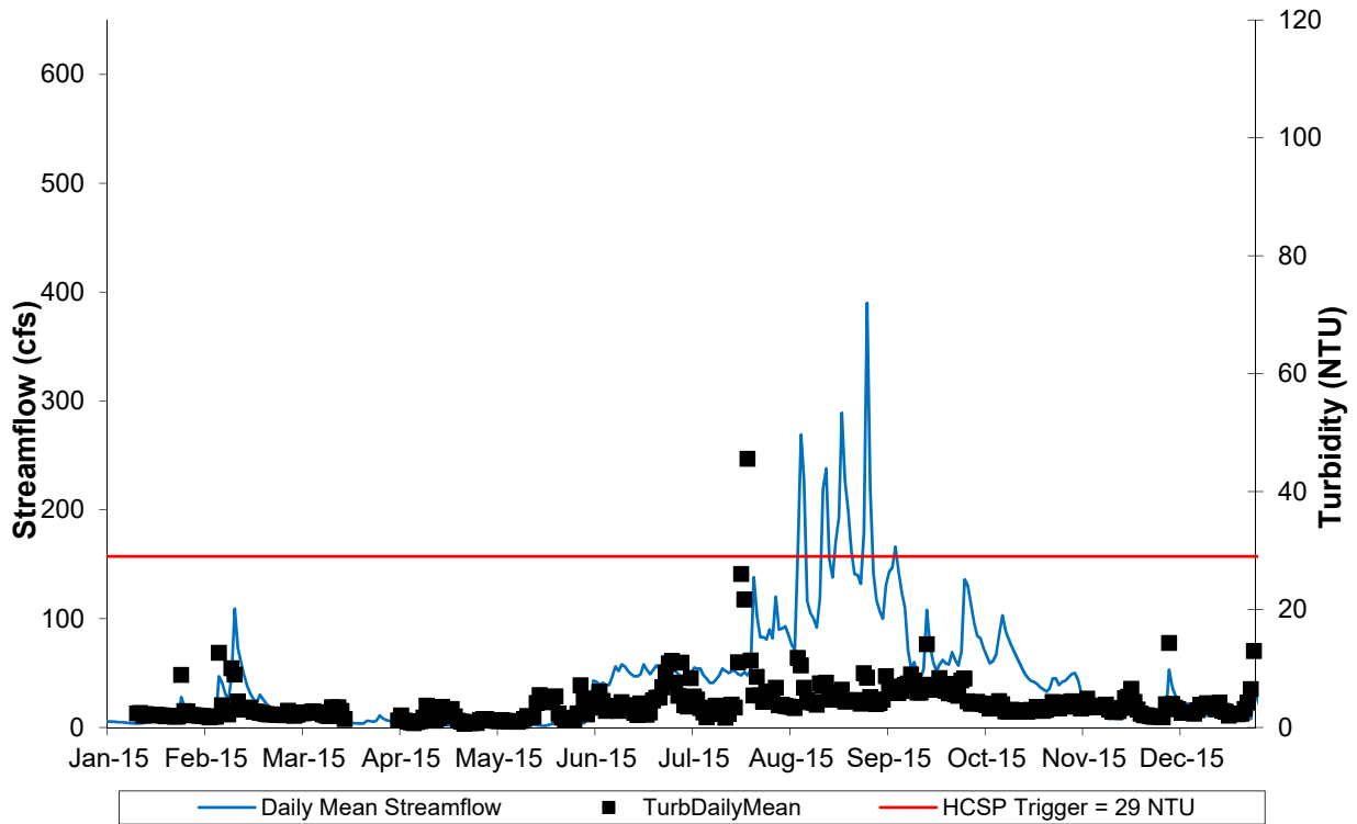
Figure 6-8. Relationship between daily mean turbidity (obtained from the continuous recorder at HCSW-1) and daily mean streamflow for 2015. Minimum detection limit = 0.1 NTU.
