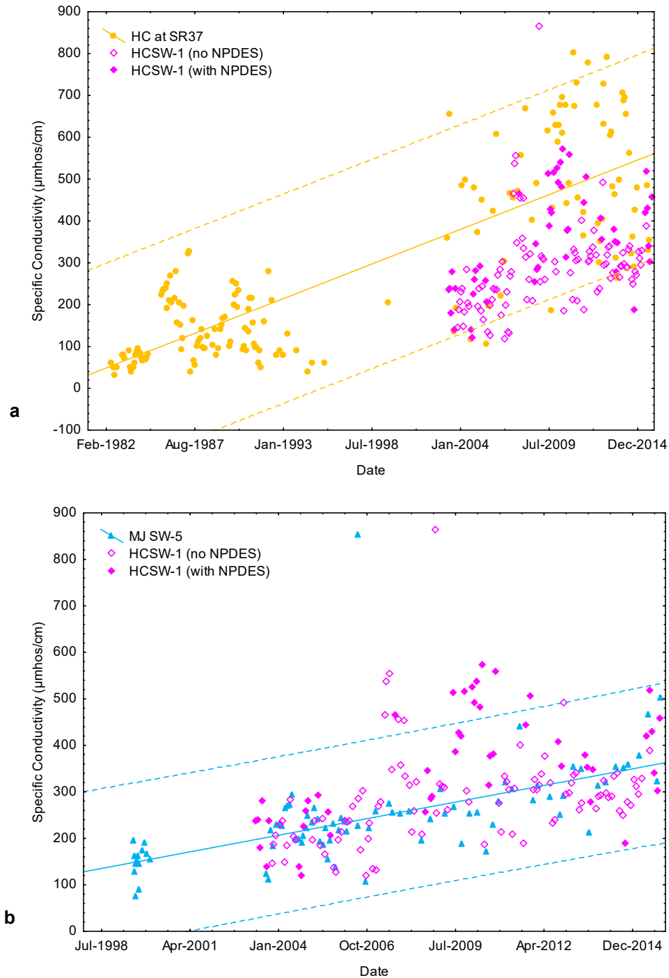
Figure I-33. HCSW-1 specific conductivity from the HCSP during periods with and without NPDES discharge, shown with 95% prediction intervals of specific conductivity at HC at SR37 (a) and MJ SW-5 (b).
