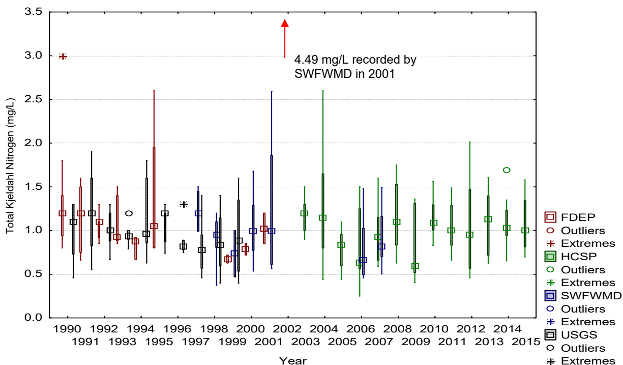
Figure C-33. HCSW-4 TKN concentrations obtained from various data sources (FDEP, SWFWMD, and USGS Data from EPA STORET and HCSP) from 1990 to 2015.
