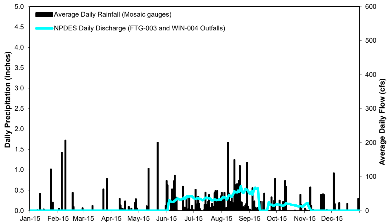
Figure 5-10. Combined Mosaic NPDES discharge and average daily rainfall in the Horse Creek watershed in 2015.
