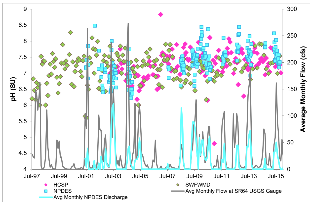
Figure I-12. HCSW-1 pH results obtained during monthly HCSP and SWFWMD water quality sampling, NPDES outfall pH results, and average monthly streamflow from USGS gauge at HCSW-1 and NPDES discharge.
