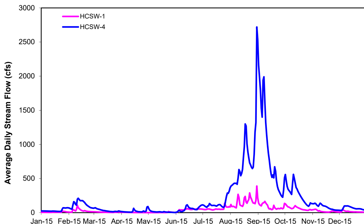
Figure 5-5. Average daily streamflow at HCSW-1 and HCSW-4 in 2015.
