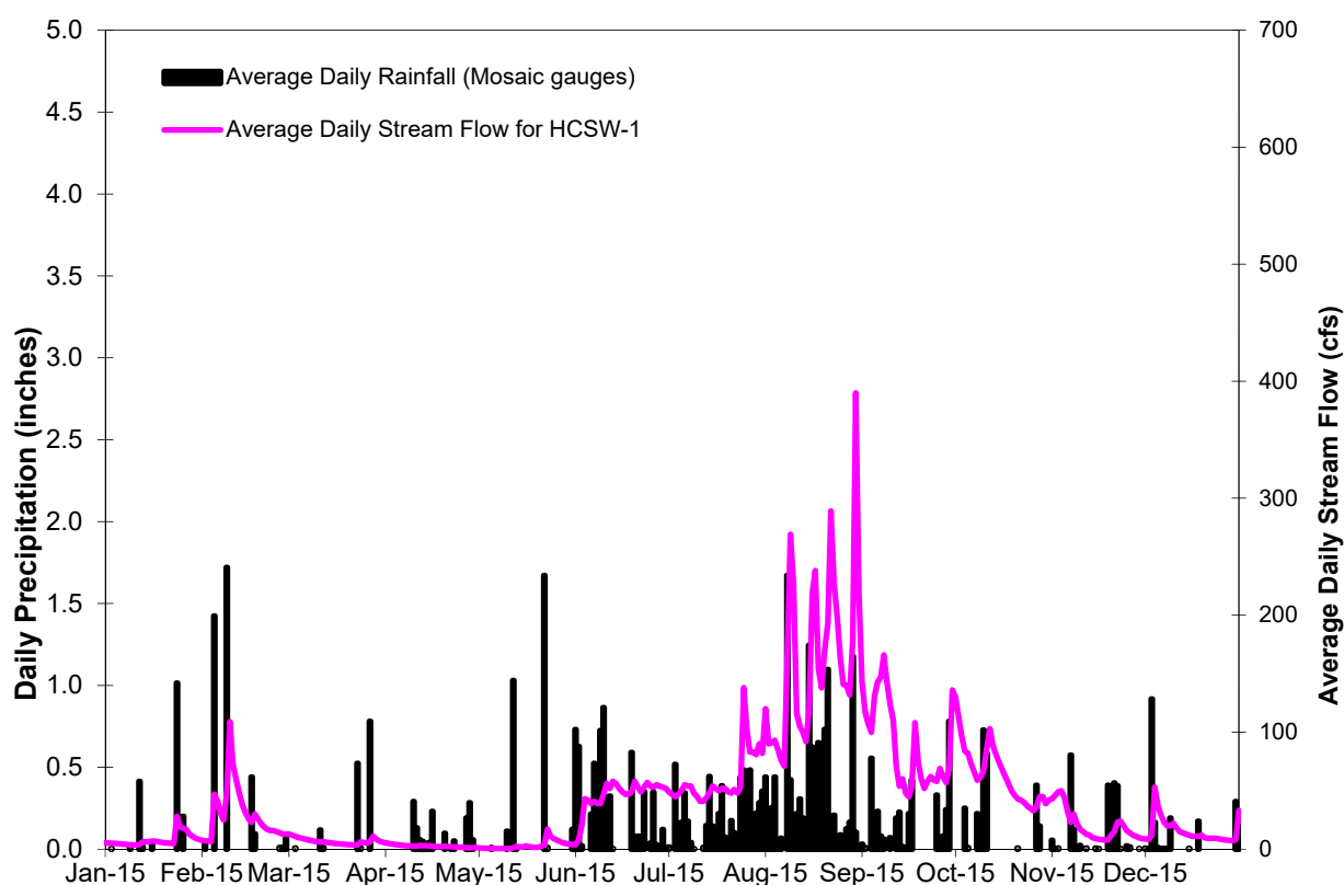
Figure 5-7. Average daily streamflow at HCSW-1 and average daily rainfall (from three Mosaic gauges 16 ) in the Horse Creek watershed in 2015.
