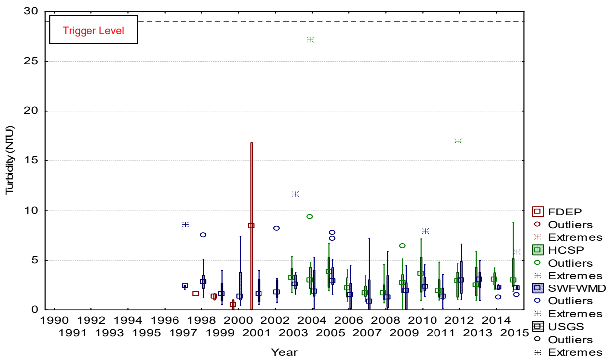
Figure C-27. HCSW-4 values of turbidity obtained from various data sources (FDEP, SWFWMD, and USGS Data from EPA STORET and HCSP) from 1990 to 2015.
