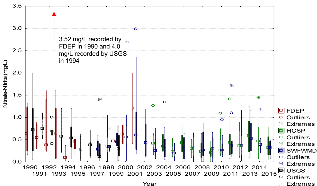
Figure C-35. HCSW-4 nitrate-nitrite concentrations obtained from various data sources (FDEP, SWFWMD, and USGS Data from EPA STORET and HCSP) from 1990 to 2015.
