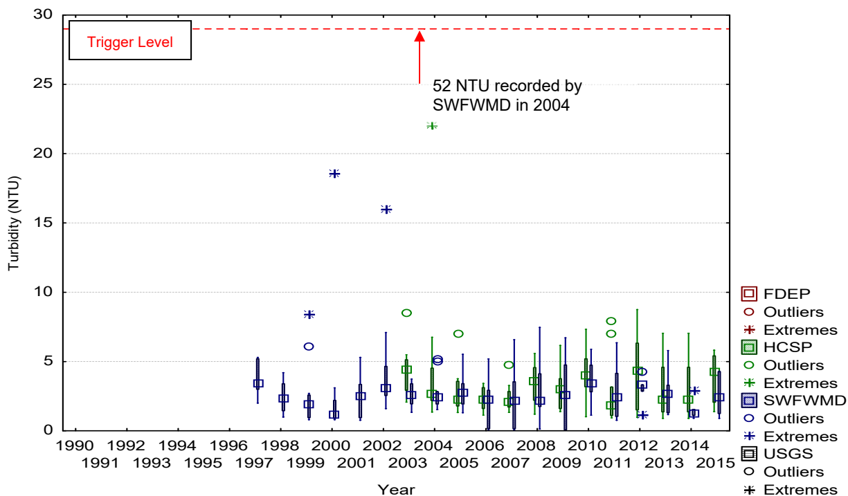
Figure C-26. HCSW-1 values of turbidity obtained from various data sources (FDEP, SWFWMD, and USGS Data from EPA STORET and HCSP) from 1990 to 2015.
