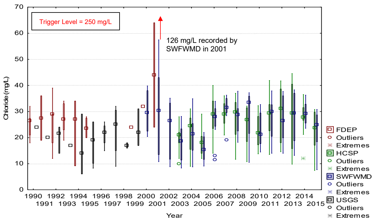
Figure C-49. HCSW-4 chloride concentrations obtained from various data sources (FDEP, SWFWMD, and USGS Data from EPA STORET and HCSP) from 1990 to 2015.
