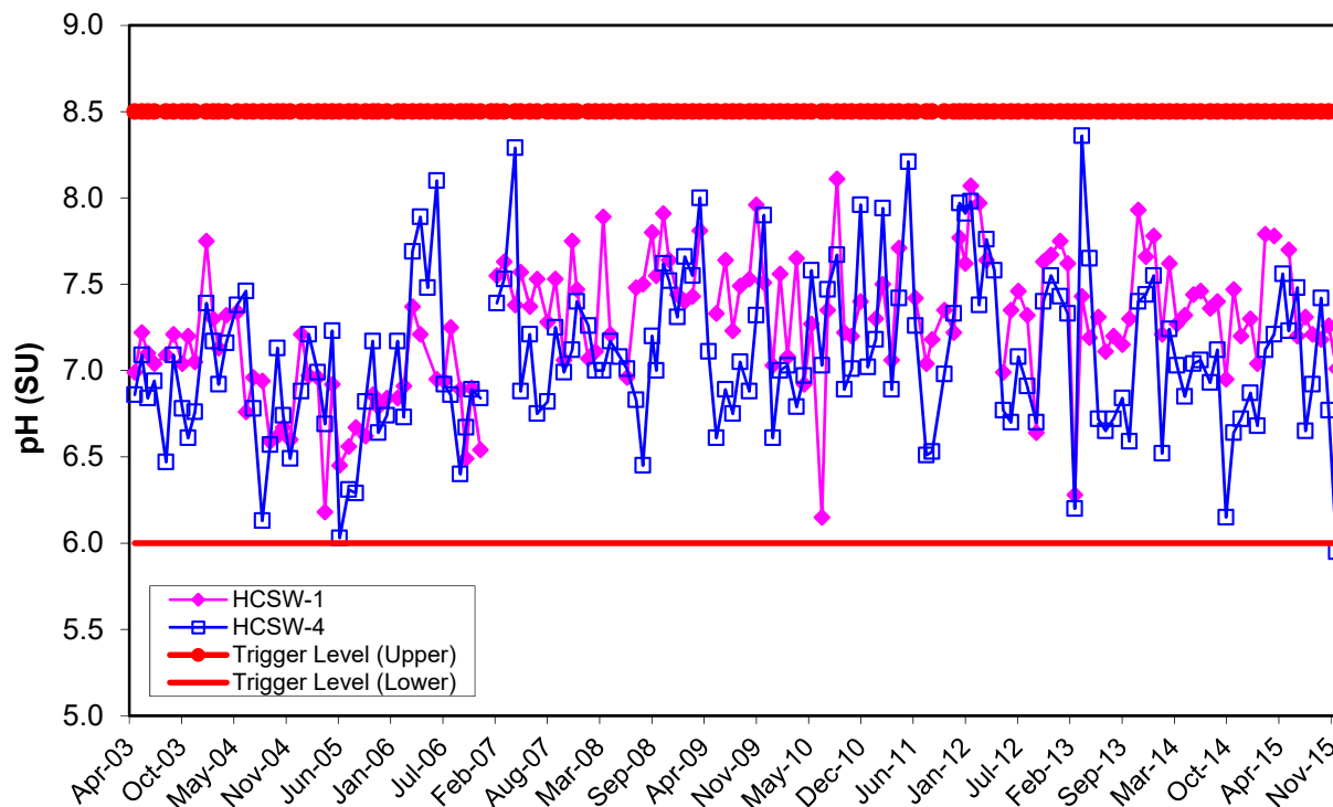
Figure I-1. Values of pH obtained during monthly HCSP water quality sampling from 2003 to 2015.
