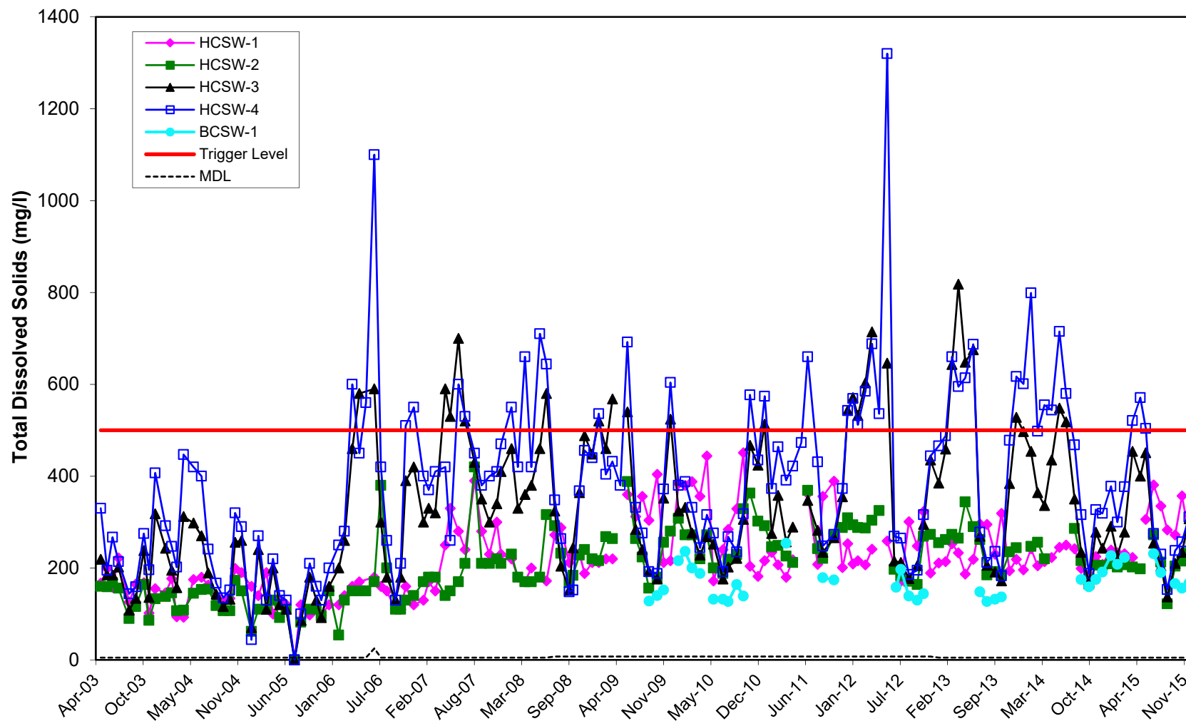
Figure C-19. Total dissolved solids concentrations obtained during monthly HCSP water quality sampling from 2003 to 2015.
