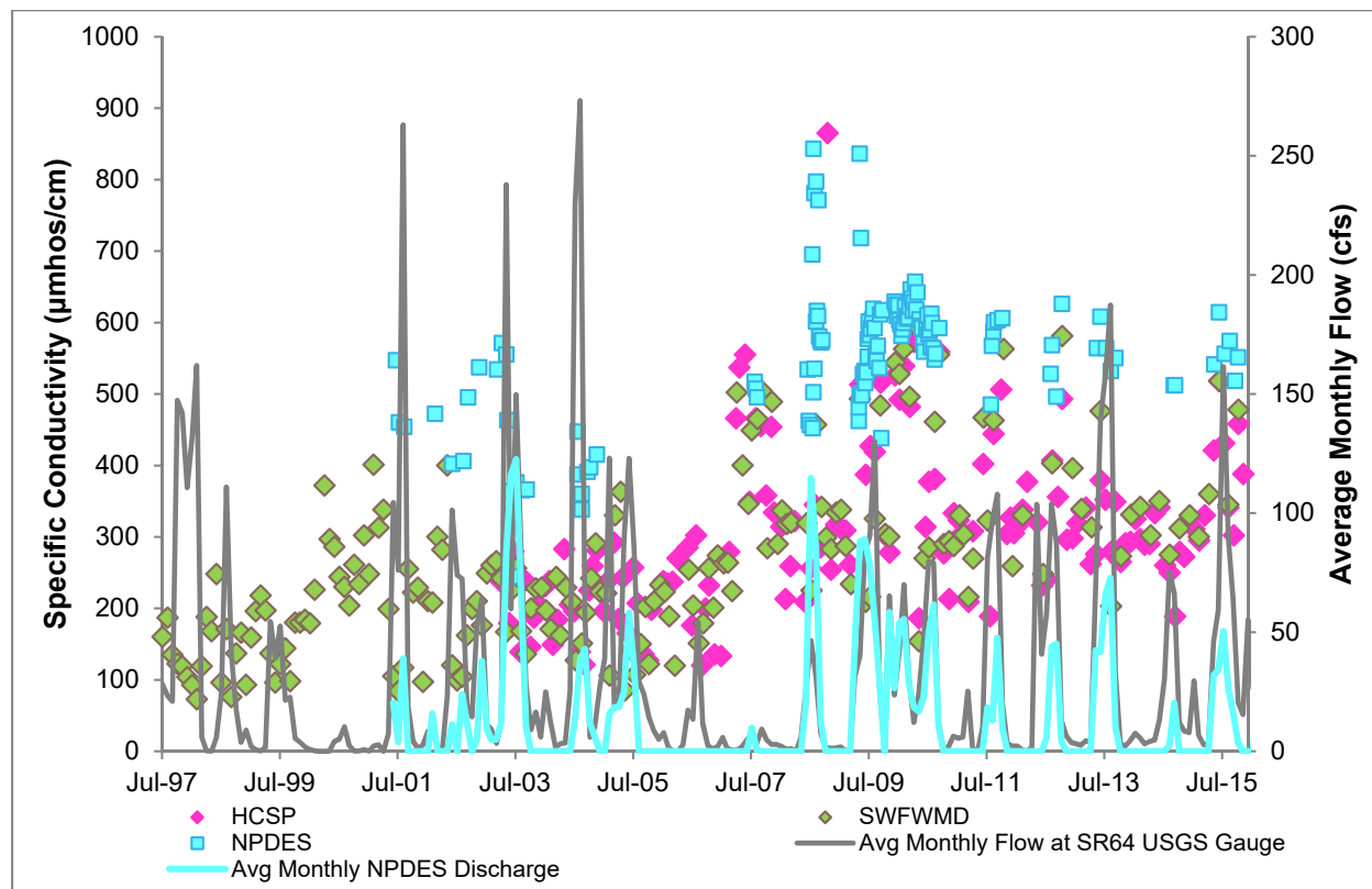
Figure I-15. HCSW-1 specific conductivity measurements obtained during monthly HCSP and SWFWMD water quality sampling, NPDES outfall specific conductivity measurements, and average monthly streamflow from USGS gauge at HCSW-1 and NPDES discharge.
