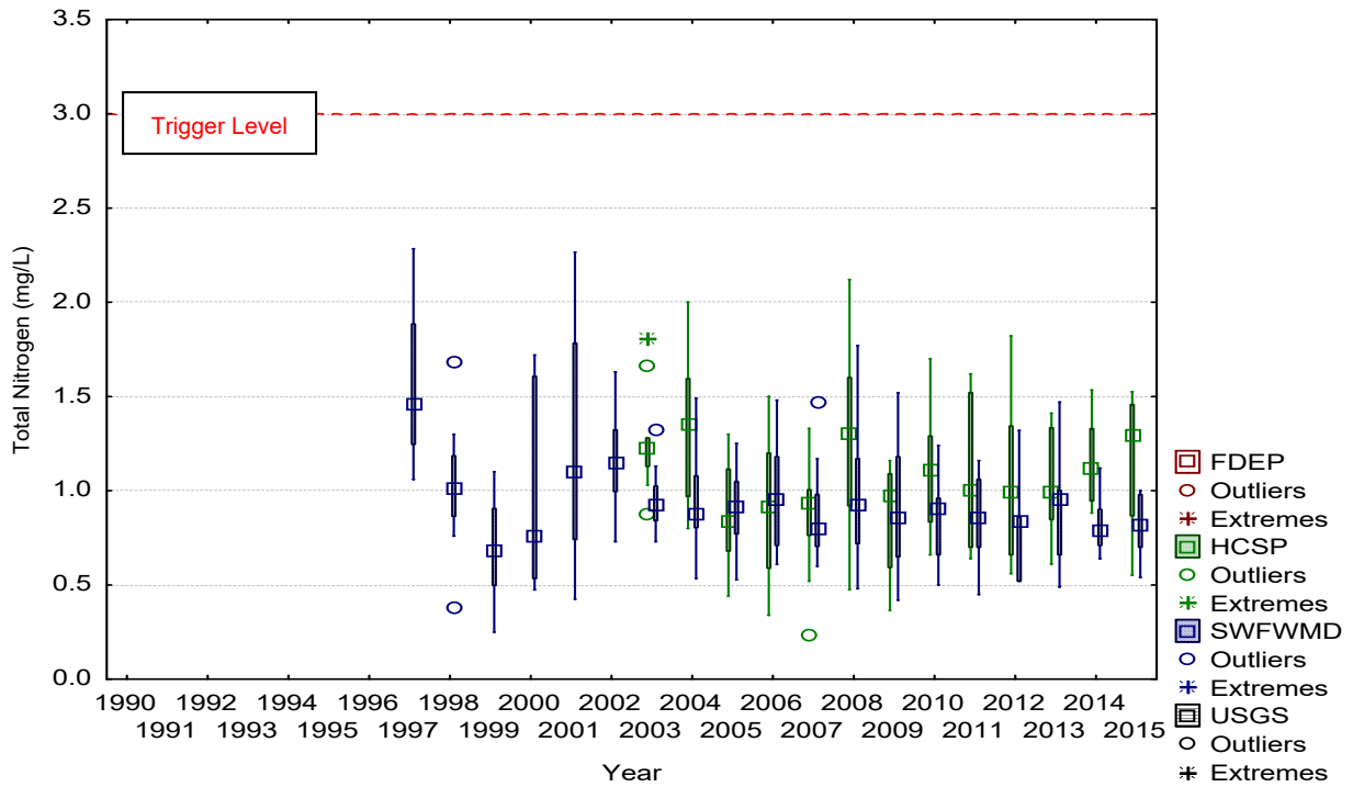
Figure C-30. HCSW-1 total nitrogen concentrations obtained from various data sources (FDEP, SWFWMD, and USGS Data from EPA STORET and HCSP) from 1990 to 2015.
