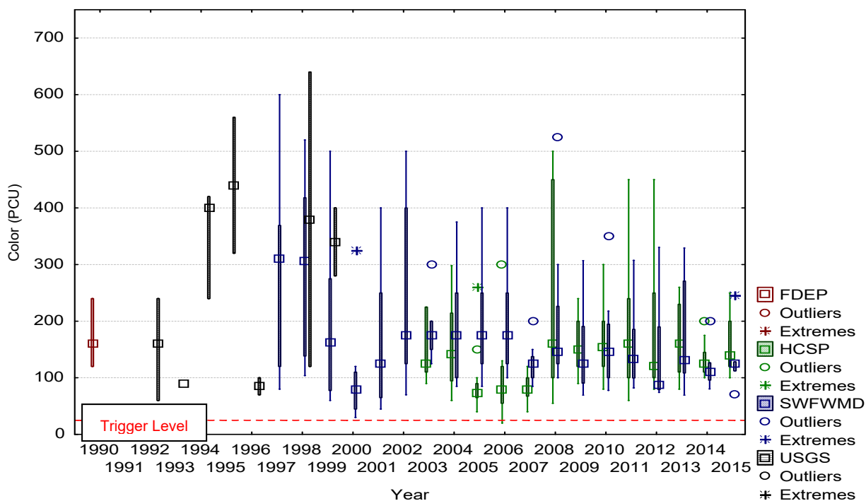
Figure C-28. HCSW-1 values of color obtained from various data sources (FDEP, SWFWMD, and USGS Data from EPA STORET and HCSP) from 1990 to 2015.
