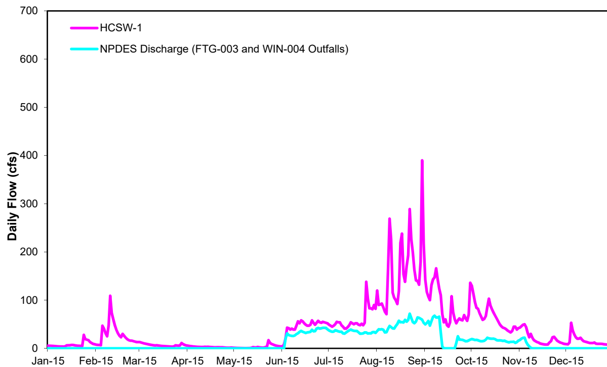
Figure 5-11. Daily streamflow at HCSW-1 and combined Mosaic NPDES discharge in 2015.
