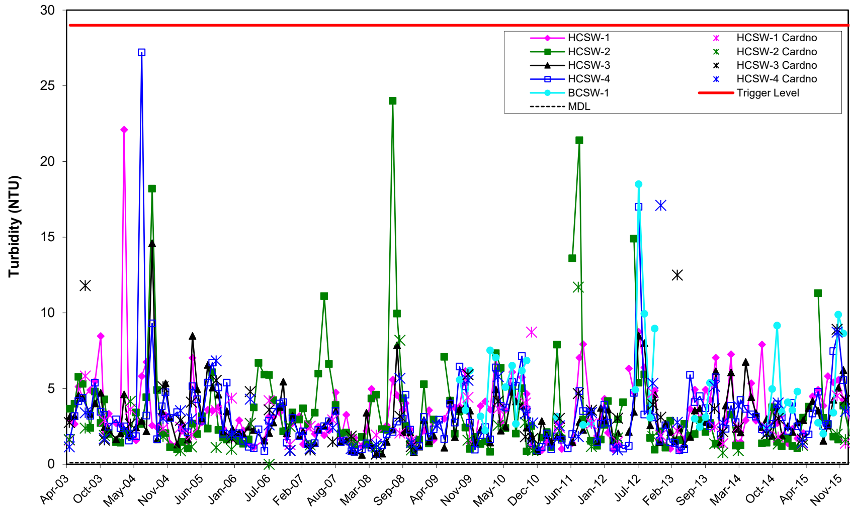
Figure C-4. Turbidity levels obtained during monthly HCSP water quality sampling and biological sampling events from 2003 to 2015.
