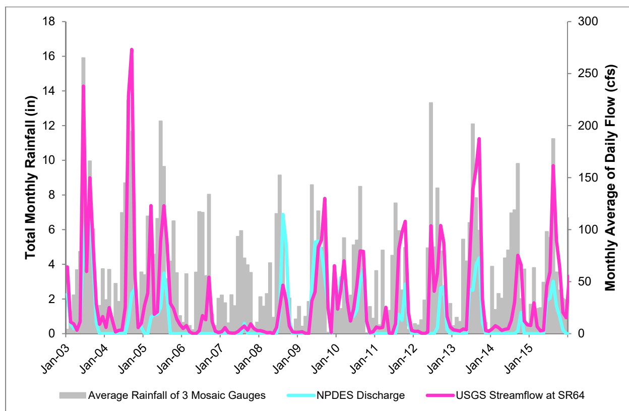
Figure I-27. Mosaic rainfall, NPDES discharge, and USGS streamflow for HCSW-1 from 2003 to 2015.
