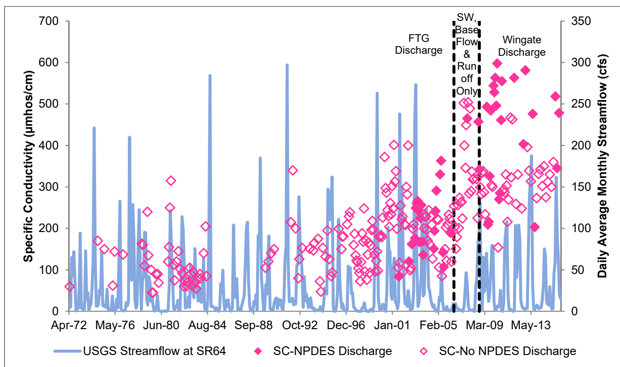
Figure I-32. Specific conductivity collected by FDEP, USGS, and SWFWMD water quality sampling from 1972 to 2015 at HCSW-1, with USGS streamflow for HCSW-1.
