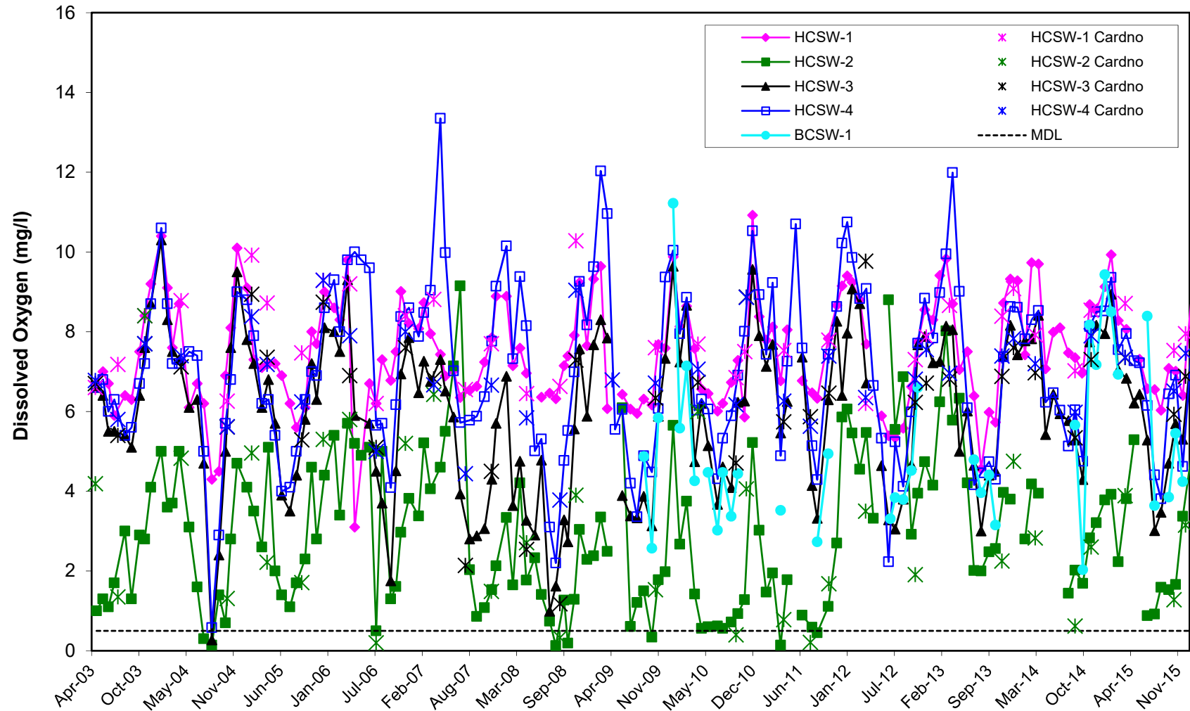
Figure C-2 Dissolved oxygen concentrations obtained during monthly HCSP water quality sampling and biological sampling events from 2003 to 2015.
