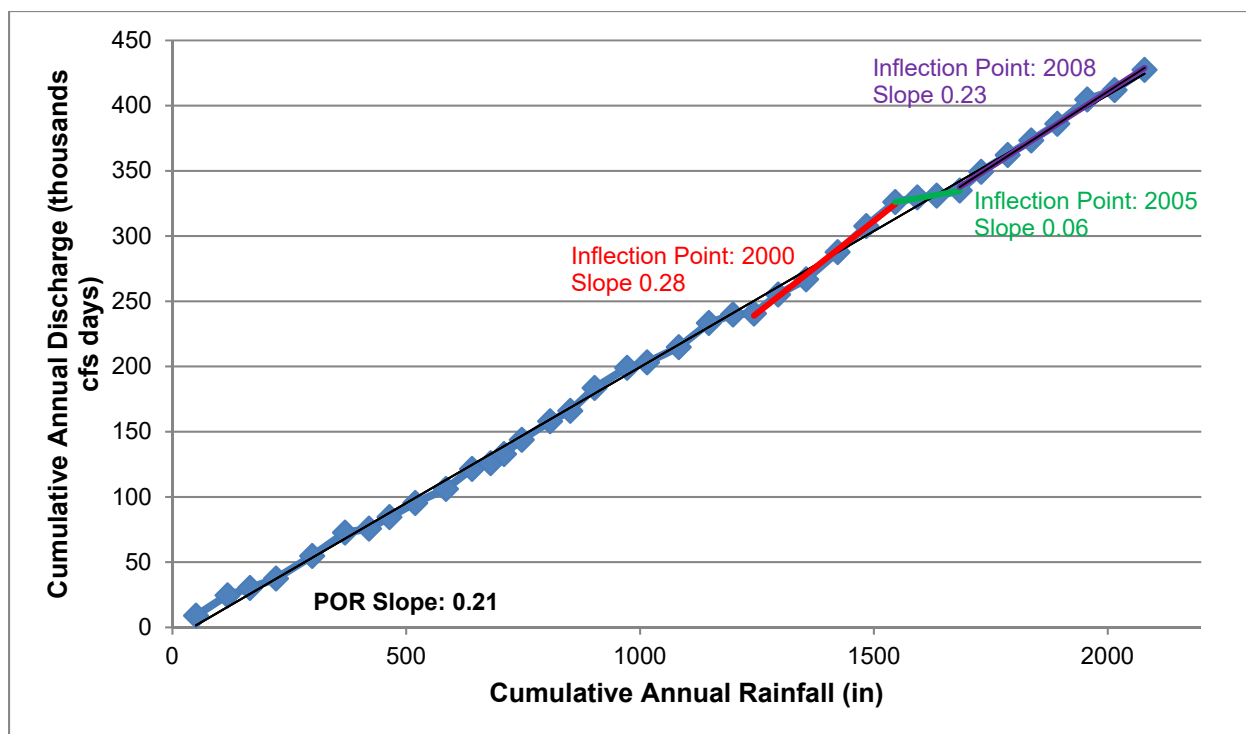
Figure 5-9. Double mass curve of cumulative daily discharge (USGS gauge at SR64) and rainfall (NOAA gauges 148 and 36) at HCSW-1 from 1978 to 2015.
