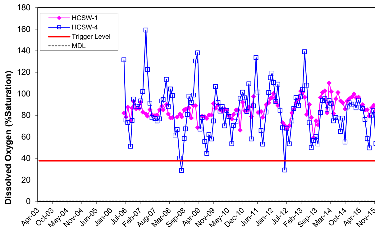
Figure I-2. Dissolved oxygen saturations obtained during monthly HCSP water quality sampling from 2003 to 2015.
