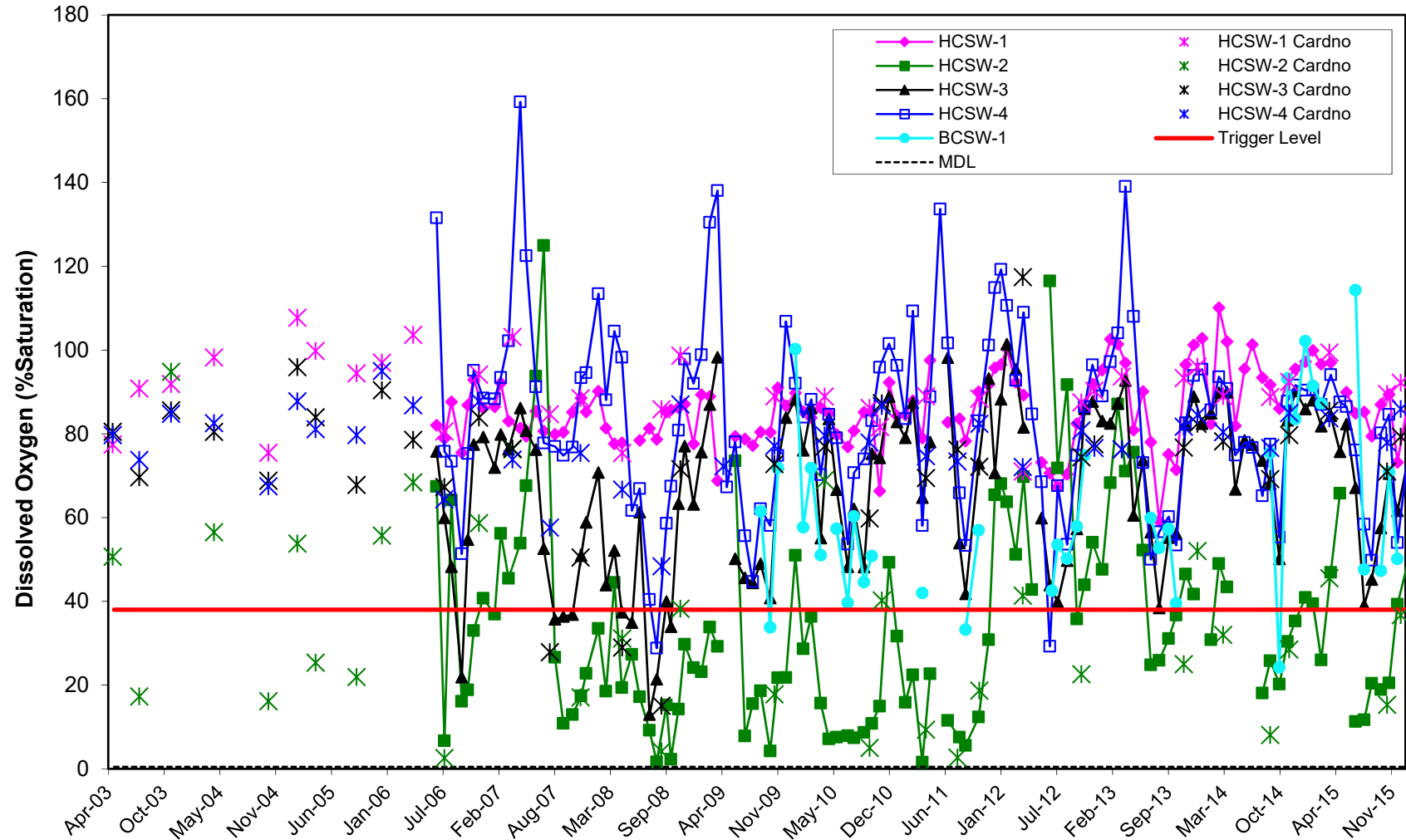
Figure C-3. Dissolved oxygen percent saturation obtained during monthly HCSP water quality sampling and biological sampling events from 2003 to 2015.
