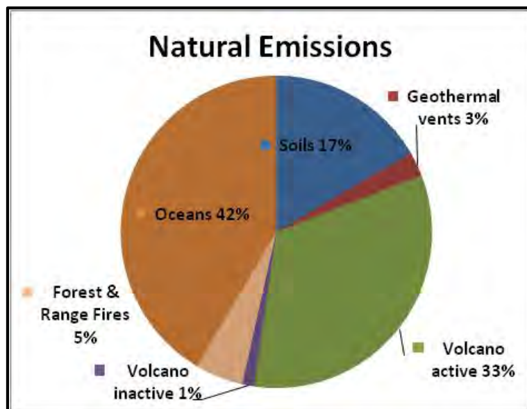
Figure 3.3. Global Natural Emissions (Derived from UNEP, 2008)
