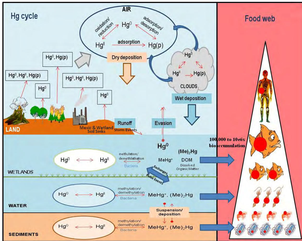
Figure 2.1. Mercury Cycling and Bioaccumulation
